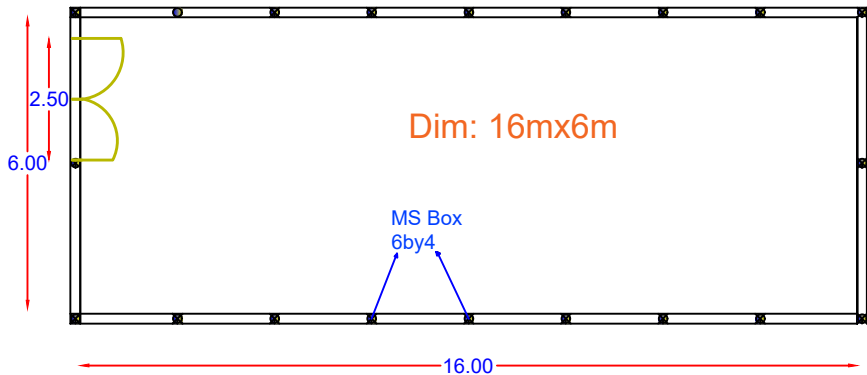
Hay store layout plan - 16mx6m
